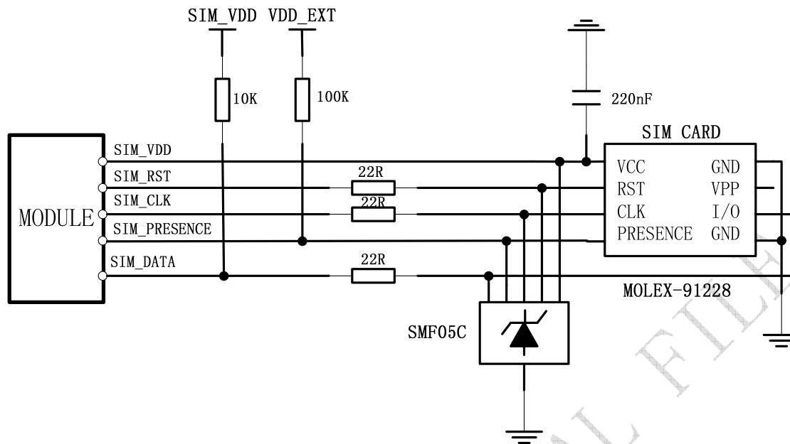
Figure 26: Reference circuit of the 8 pins SIM card
