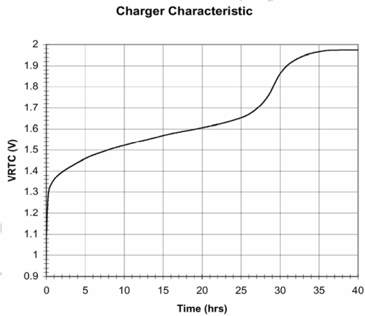
Figure 16: Seiko TS621 Charge Characteristic
