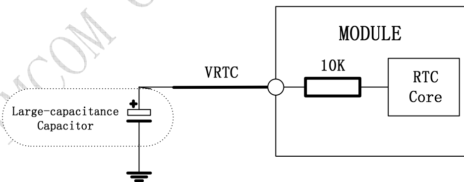
Figure 13: RTC supply from capacitor
