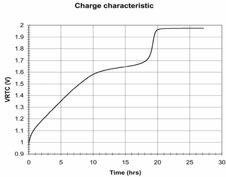
Figure 15: Maxell TC614 Charge Characteristic
